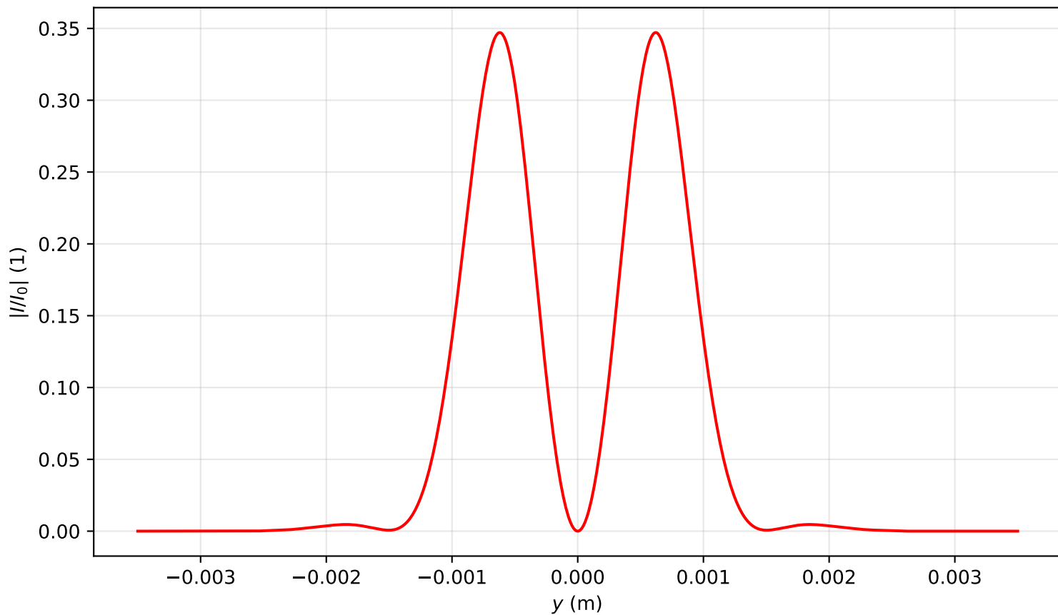
Intensity profile I(x=0, y, z=1.831)/I_0 , P_{in}=4.0P_{cr} , artificial time
